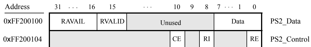
Figure 43. PS/2 port registers.
