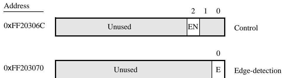
Figure 42. The video-in port programming interface.
