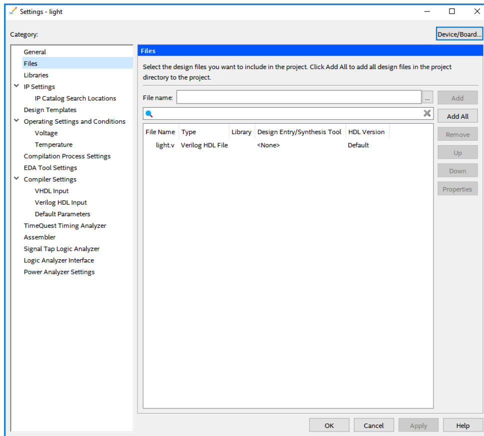
Figure 17. Settings window.
