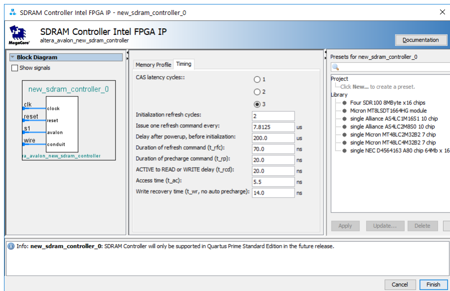
Figure 5. SDRAM Timings
