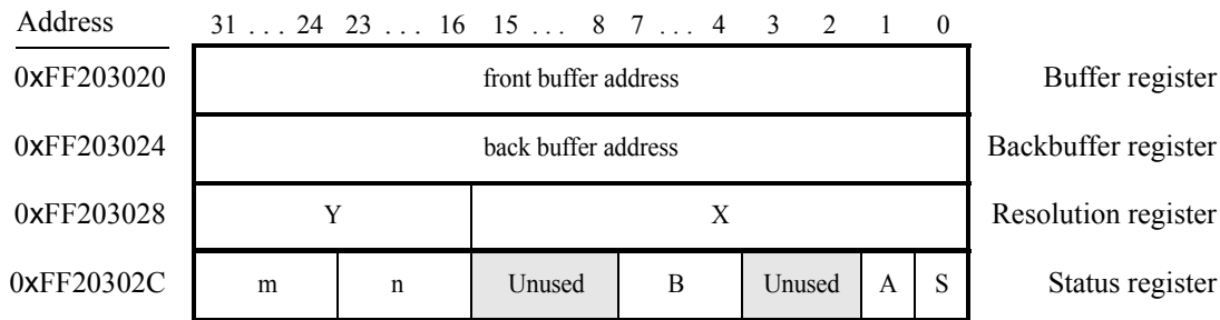
Figure 3: Pixel buffer controller registers.
