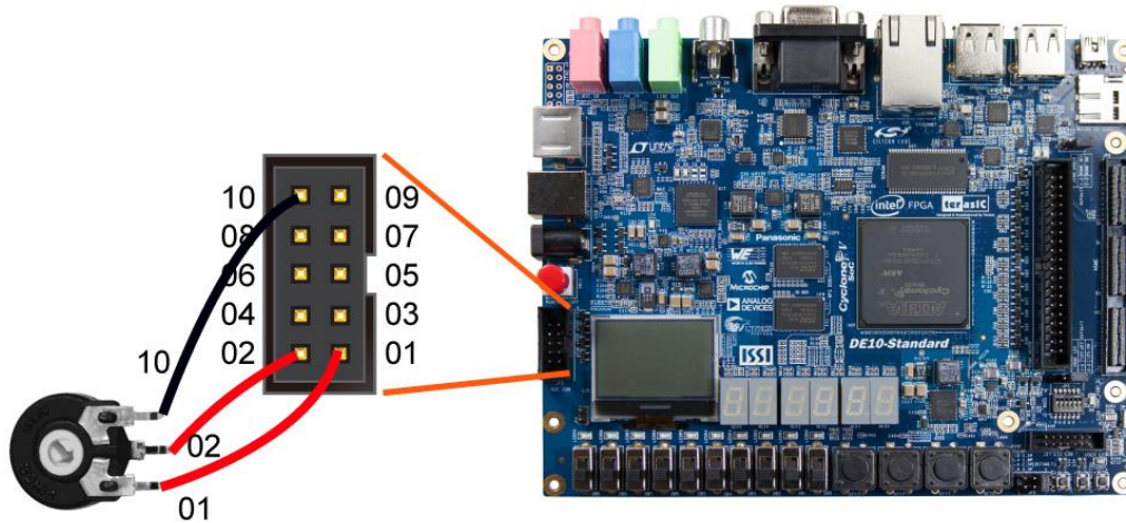
Figure 5-23 Hardware setup for the ADC reading demonstration
