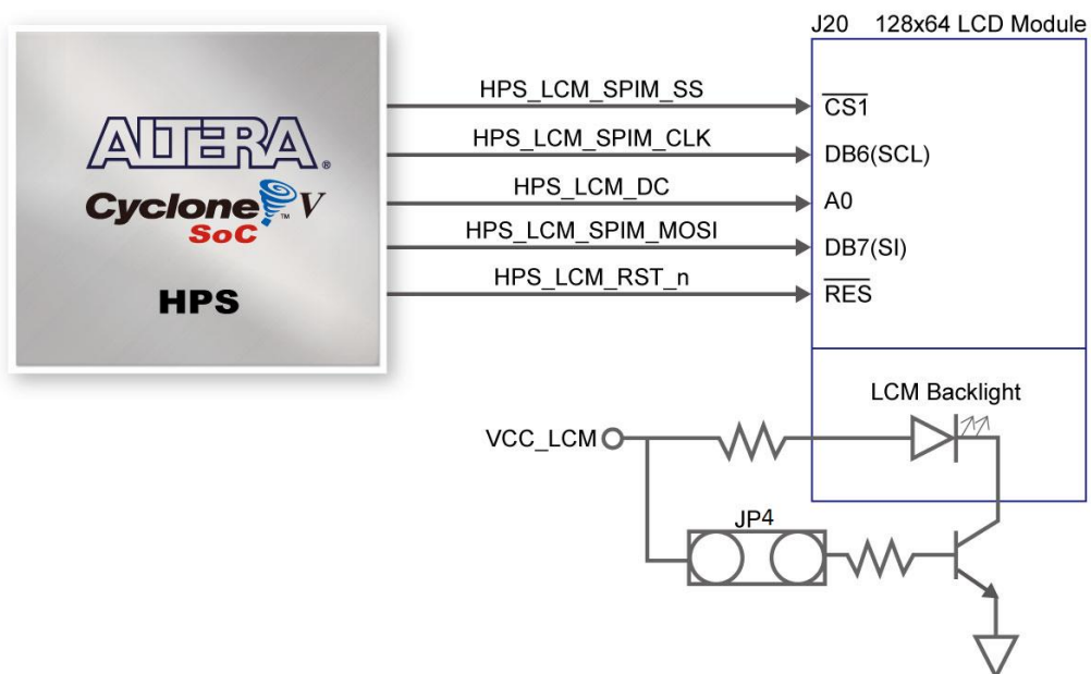
Figure 3-39 Connections between Cyclone V SoC FPGA and LCD Module
