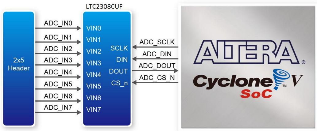
Figure 3-30 Connections between the FPGA, 2x5 header, and the A/D converter
