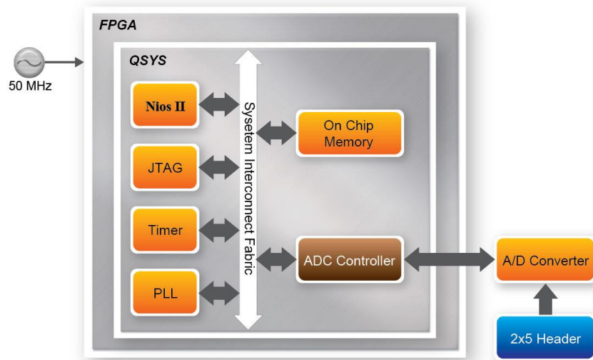
Figure 5-19 Block diagram of ADC reading
