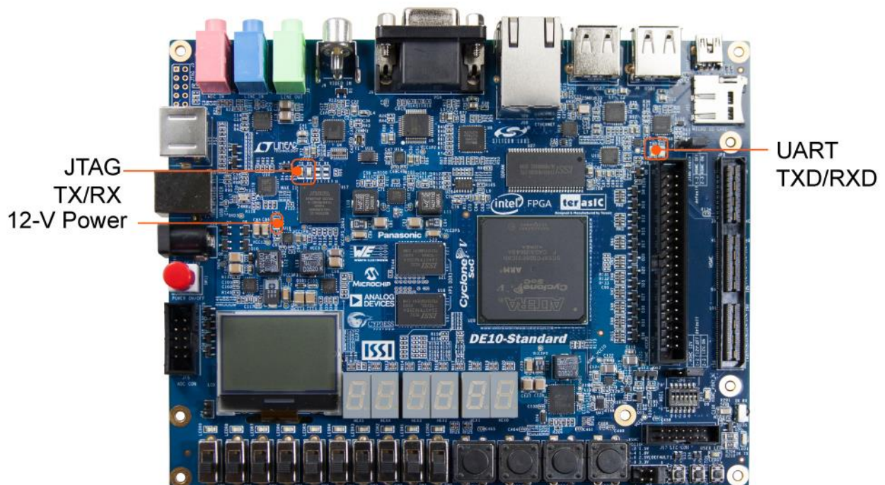
Figure 3-10 LED Indicators on DE10-Standard
