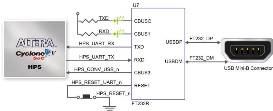
Figure 3-32 Connections between the HPS and FT232R Chip
