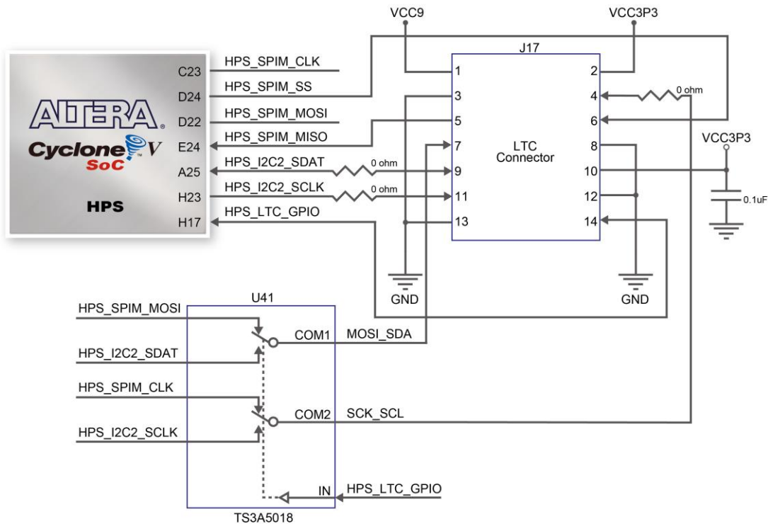
Figure 3-36 Connections between the HPS and LTC connector
