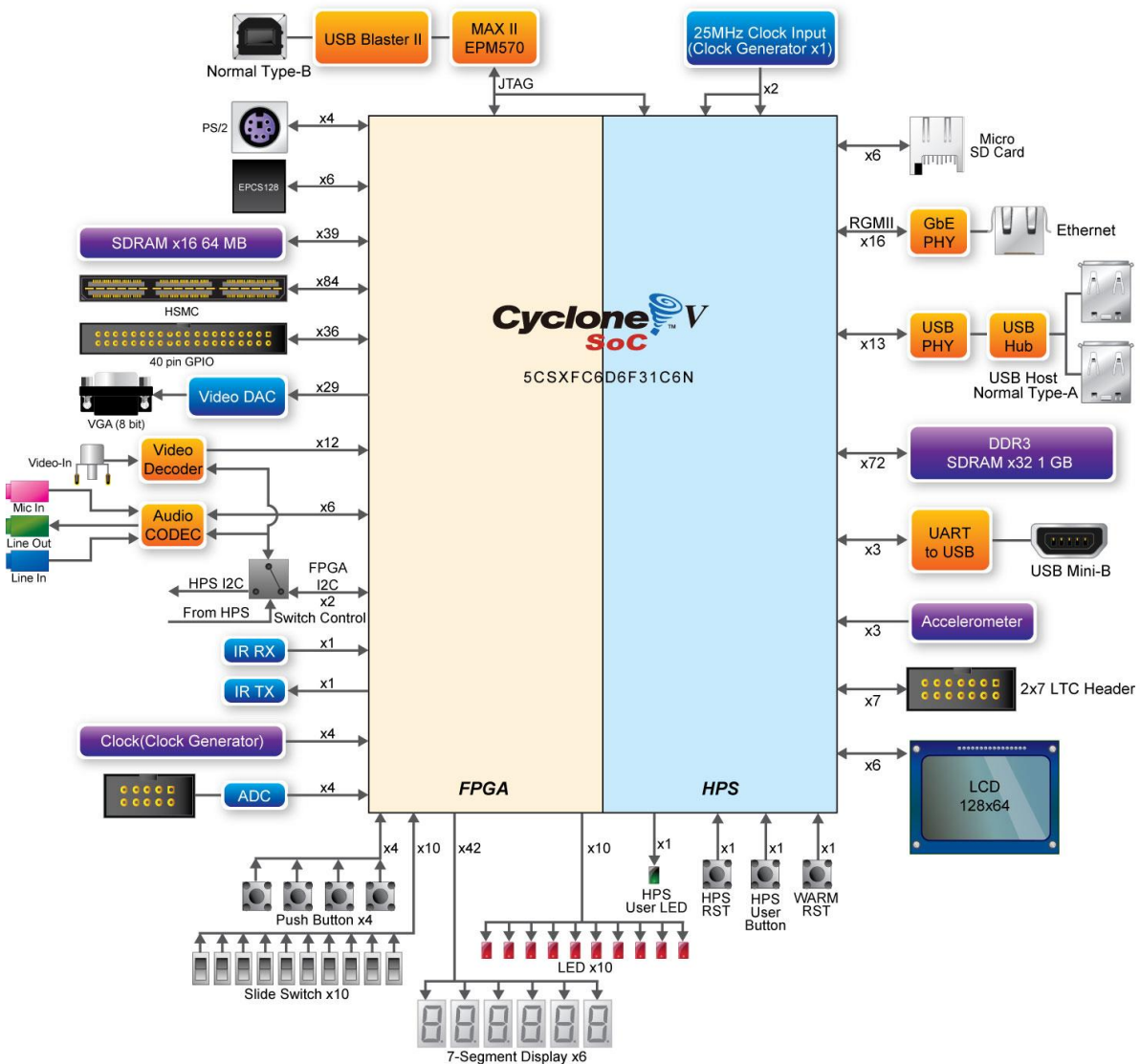
Figure 2-3 Block diagram of DE10-Standard
