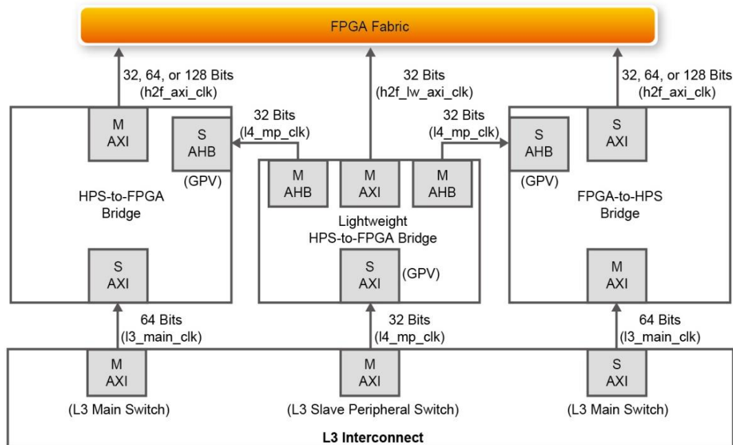
Figure 7-1 AXI Bridge Block Diagram
