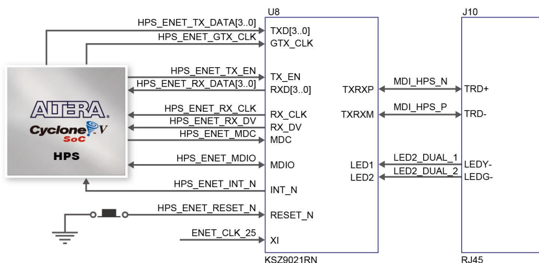
Figure 3-31 Connections between the HPS and Gigabit Ethernet
