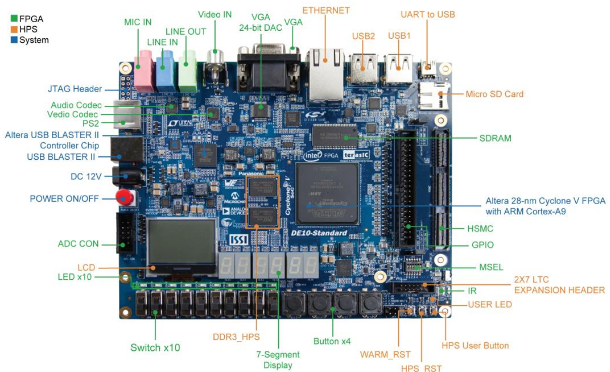
Figure 2-1 DE10-Standard development board (top view)
