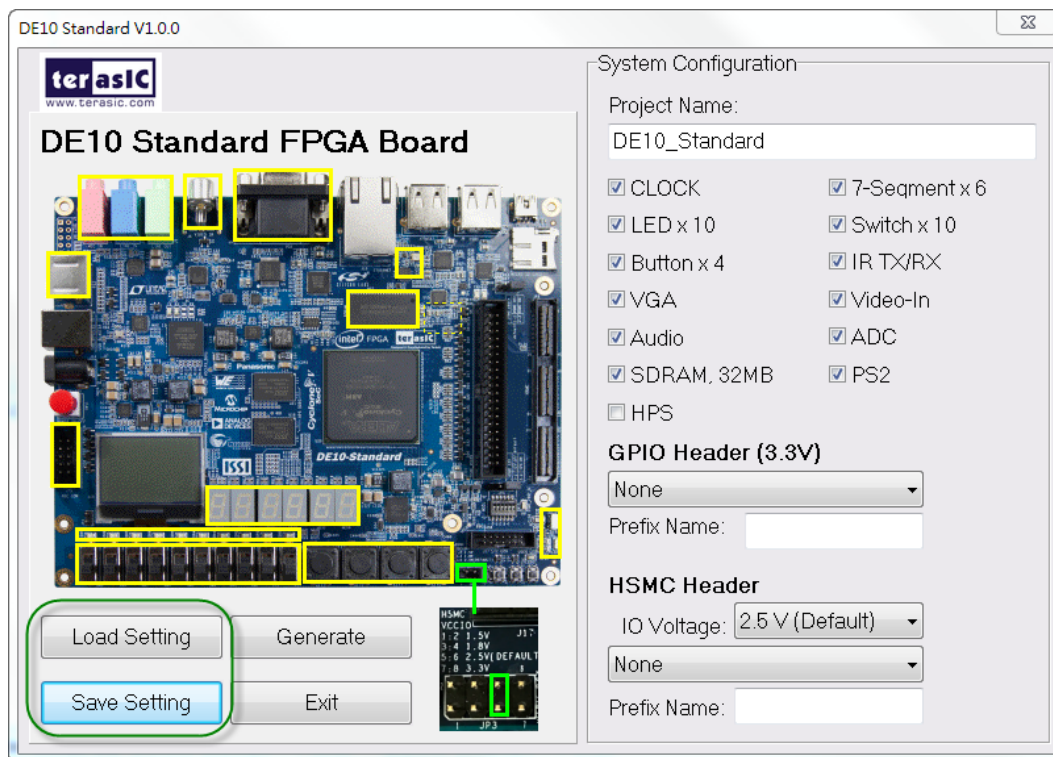
Figure 4-6 Project Settings
