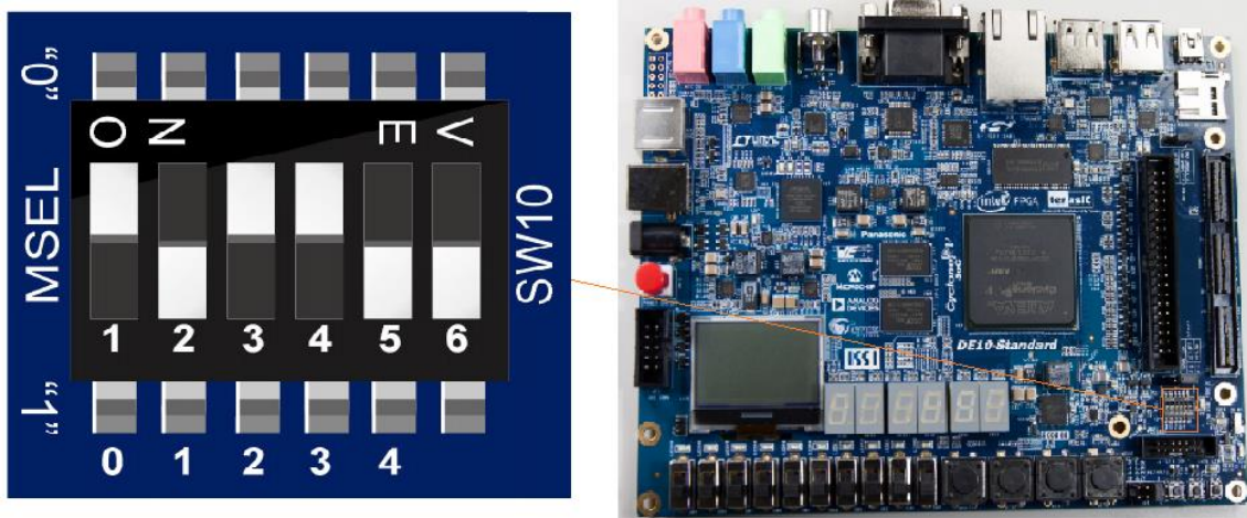
Figure 3-1 DIP switch (SW10) setting of Active Serial (AS) mode on DE10-Standard board
