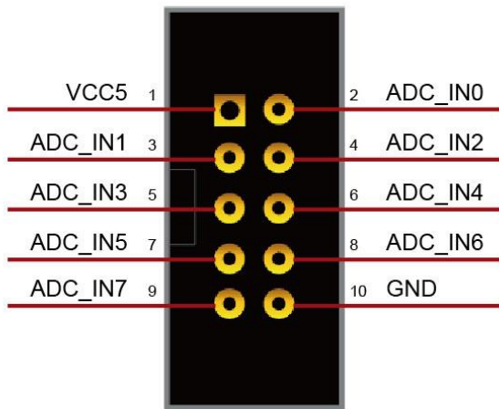
Figure 3-29 Signals of the 2x5 Header
