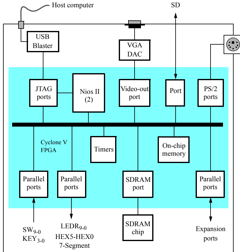
Figure 1. Block diagram of the DE0-CV Computer.
